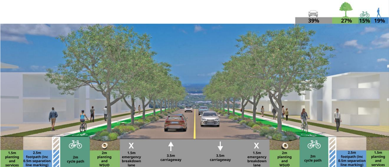
Figure 6: Cross section — 2 lane sub-arterial / arterial
